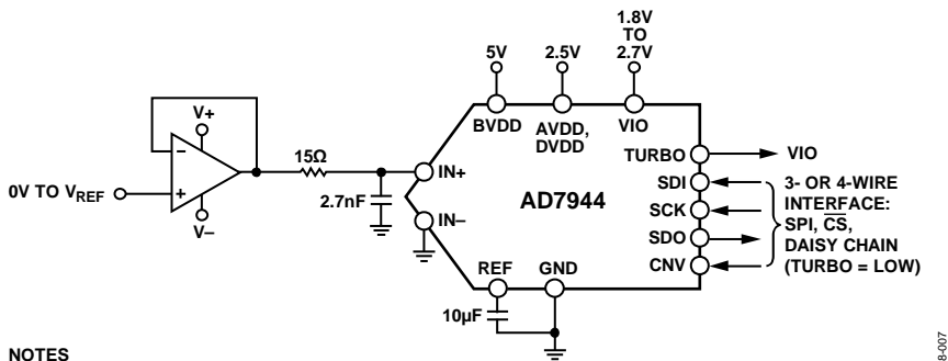
Figure 23. Typical Application Diagram with Multiple Supplies
