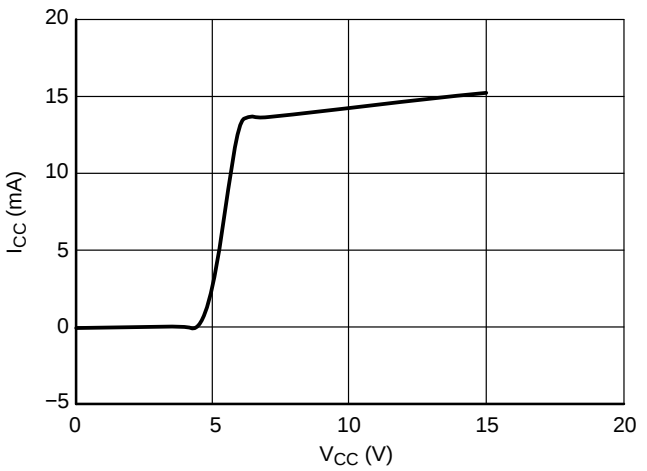
Figure 38. Power Supply Current in Working Mode vs. Power Supply Voltage – V CC
