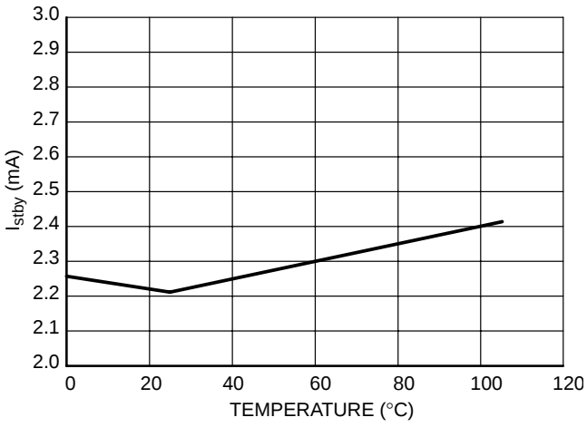
Figure 35. Power Supply Current in Standby Mode vs. Temperature
