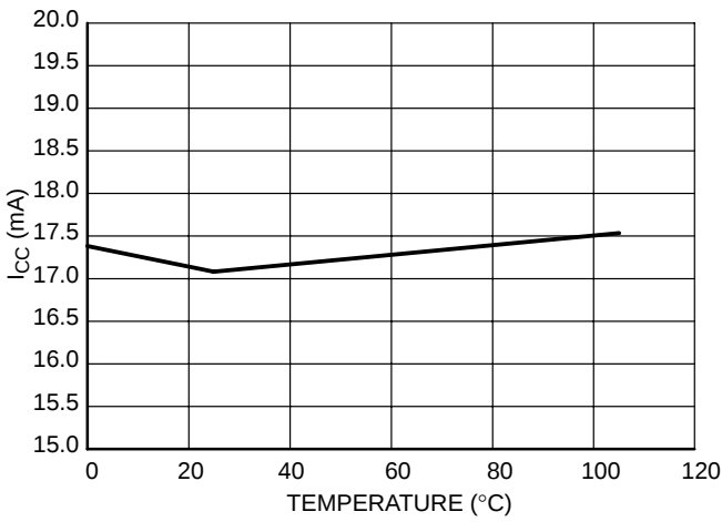
Figure 37. Power Supply Current in Working Mode vs. Temperature
