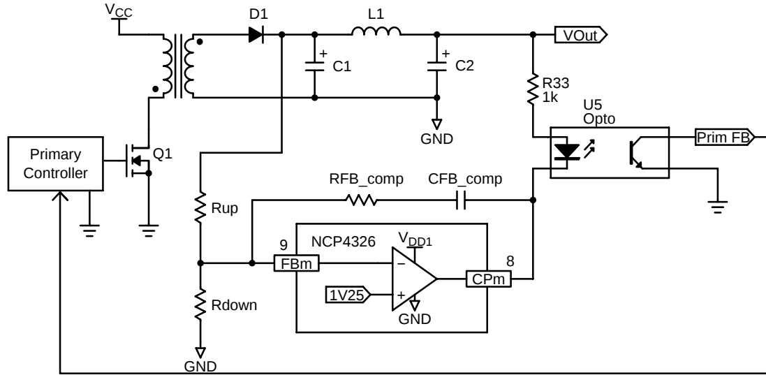
Figure 53. Primary Feedback Connection
