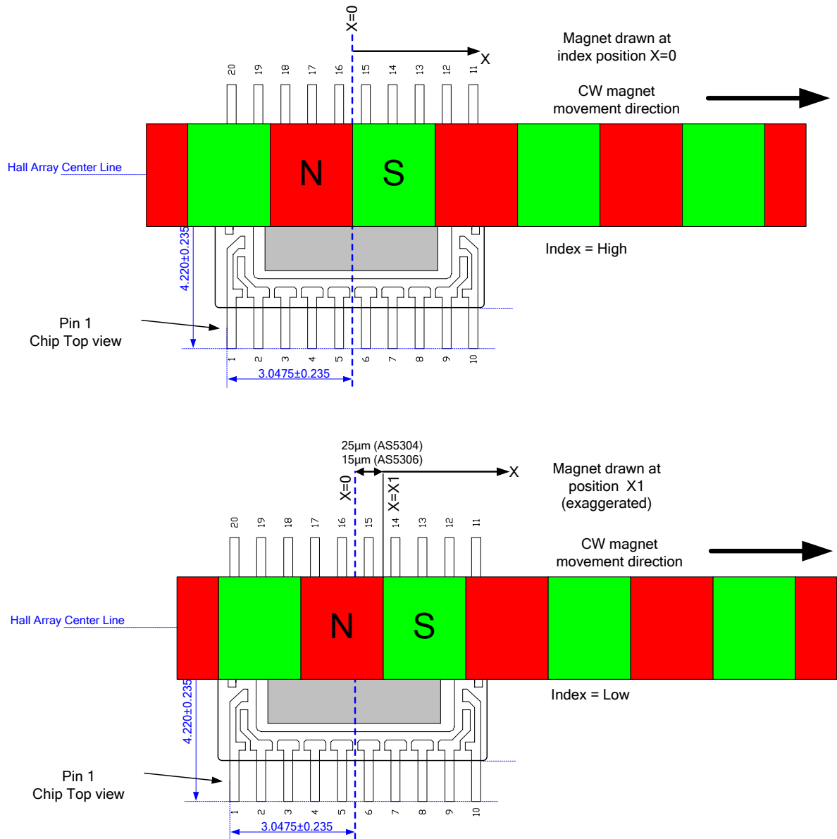
Figure 7: Magnet placement for index pulse generation
