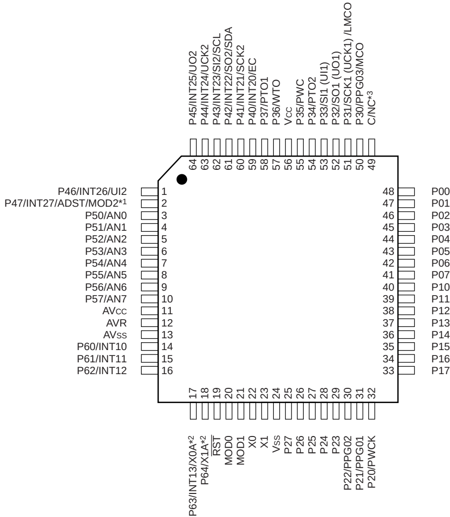
(TOP VIEW)
