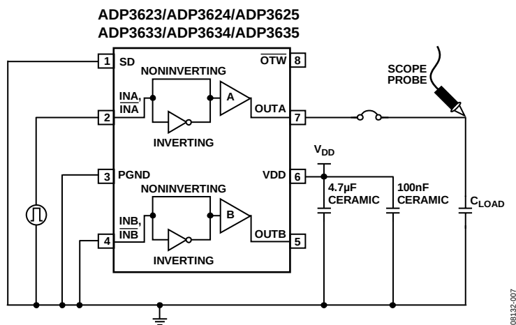
Figure 20. Test Circuit
