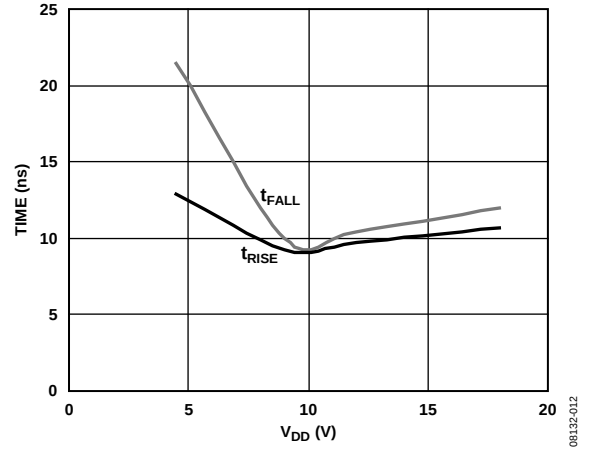
Figure 13. Rise and Fall Times vs. V_{DD}
