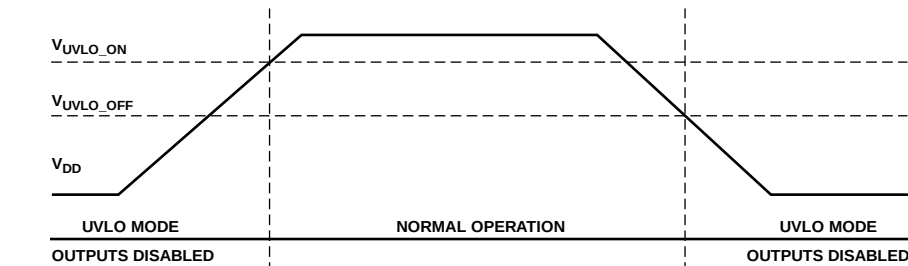
Figure 5. UVLO Function
