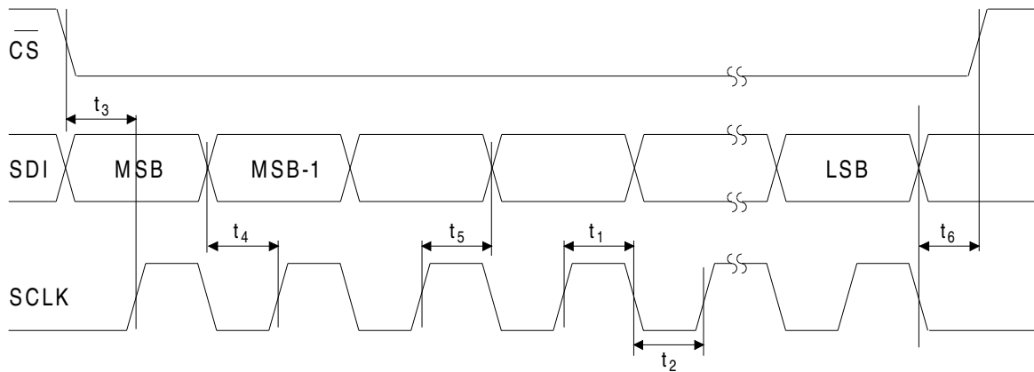
Figure 2. SDI Write Timing (Not to Scale)
