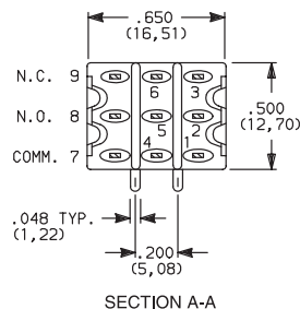
PC MOUNTING
