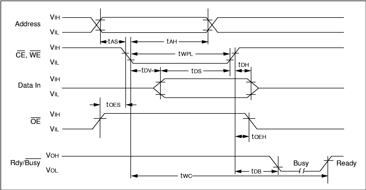
FIGURE 1-2: PROGRAMMING WAVEFORMS
