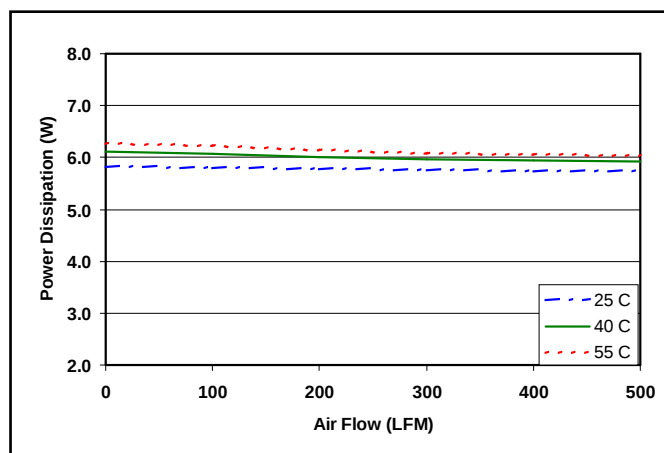
Figure 6: Power dissipation at 80% load and 50/50 voltage split (7.3A load on 3.3V and 4.8A load on 5.0V) versus airflow rate for ambient air temperatures of 25°C, 40°C and 55°C (nominal input voltage).
