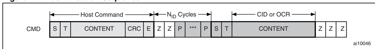
Figure 17. Identification Sequence
