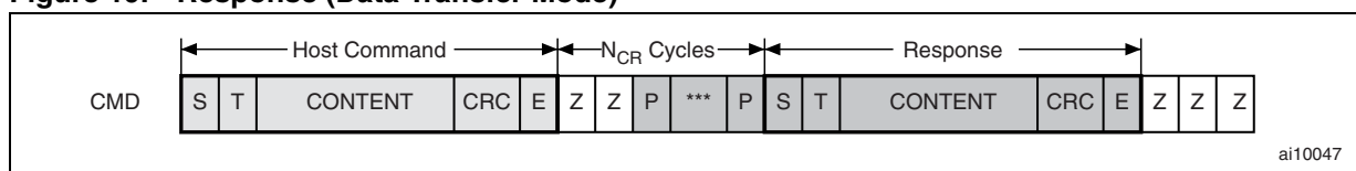
Figure 19. Response (Data Transfer Mode)
