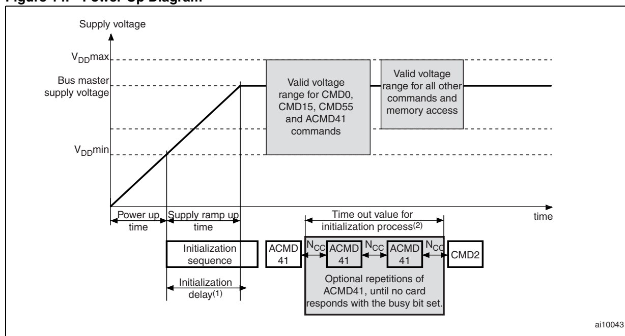
Figure 14. Power-Up Diagram
