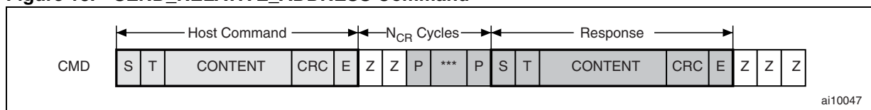
Figure 18. SEND_RELATIVE_ADDRESS Command
