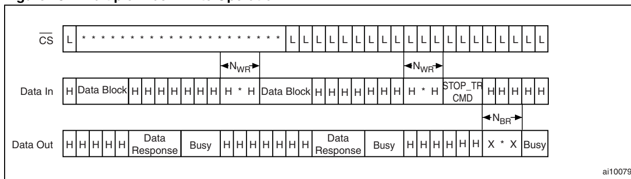
Figure 45. Multiple Block Write Operation
