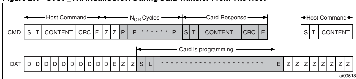
Figure 27. STOP TRANSMISSION During Data Transfer From The Host
