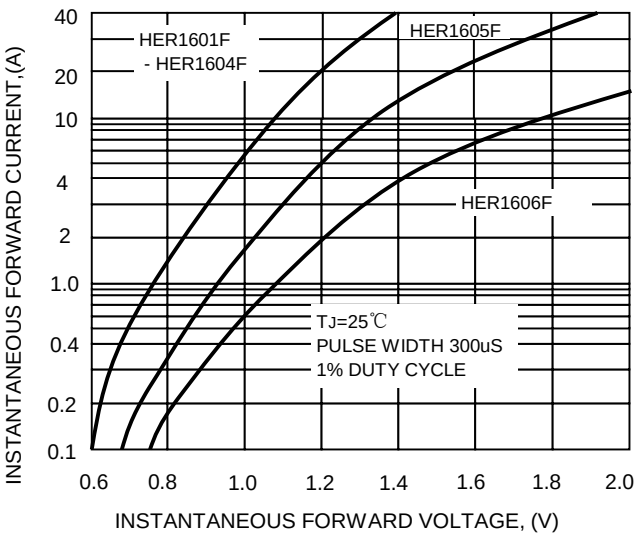
FIG.4-TYPICAL INSTANTAEIOUS FORWARD CHARACTERISTICS
