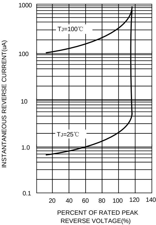
FIG.2-TYPICAL REVERSE CHARACTERISTICS
