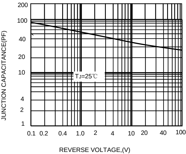
FIG.5-TYPICAL JUNCTION CAPACITANCE
