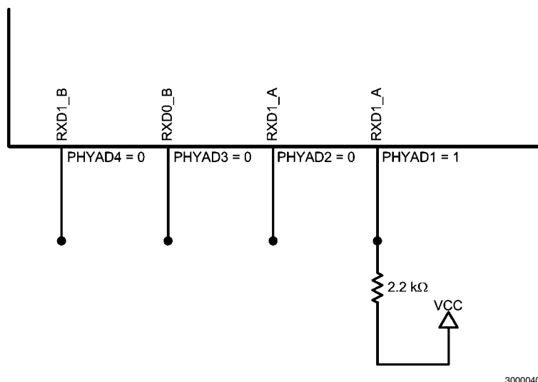
FIGURE 1. PHYAD Strapping Example
