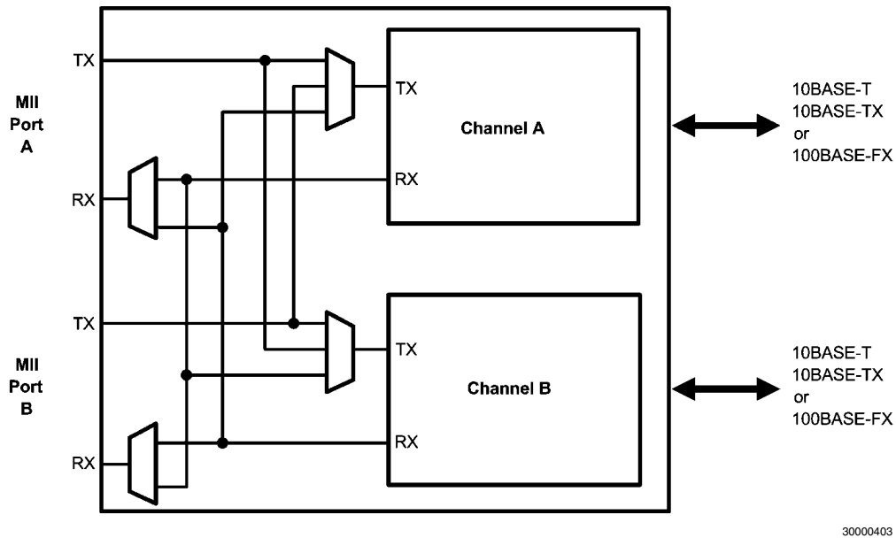
FIGURE 3. MII Port Mapping
