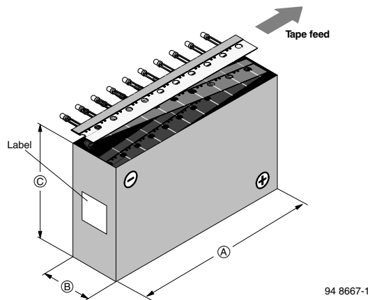
Figure 10. Tape Direction
