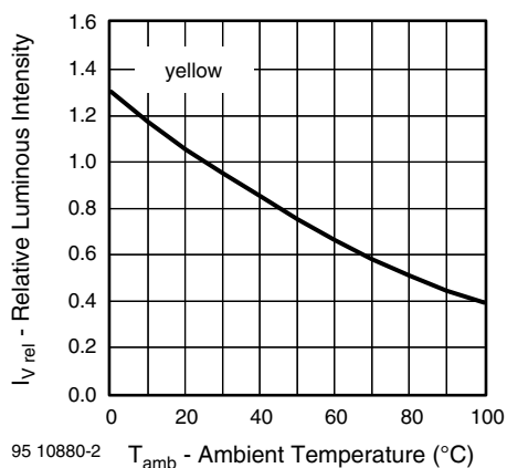
Figure 7. Relative Luminous Intensity vs. Ambient Temperature
