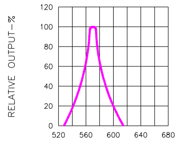
Fig.2 SPECTRAL RESPONSE
