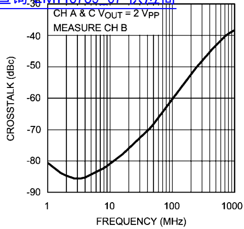
查询"LMH6739_07"供应商 Crosstalk vs. Frequency
