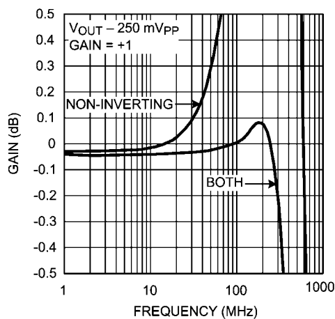
Gain Flatness, Dual Input Buffer
