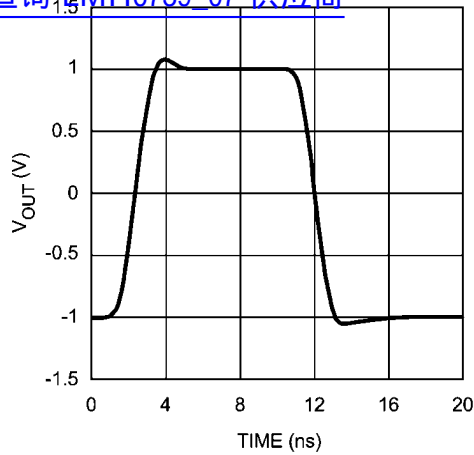
Pulse Response 查询"LMH6739_07"供应商
