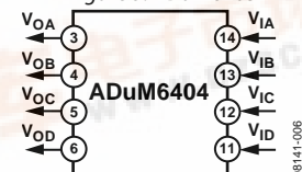
Figure 6. ADuM6404
