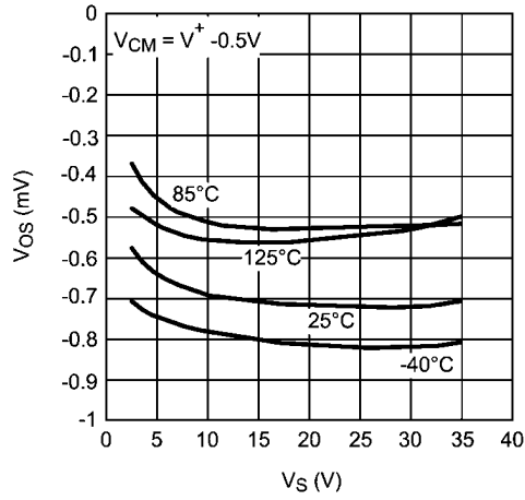
V OS vs. V S (Unit 2)
