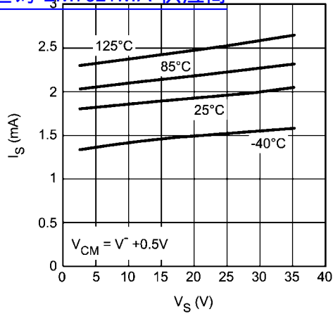
I_S vs. V_S (LM7322) 查询"LM7321MA"供应商
