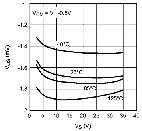
V OS vs. V S (Unit 1)
