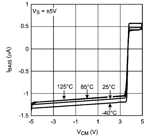
I BIAS vs. V CM
