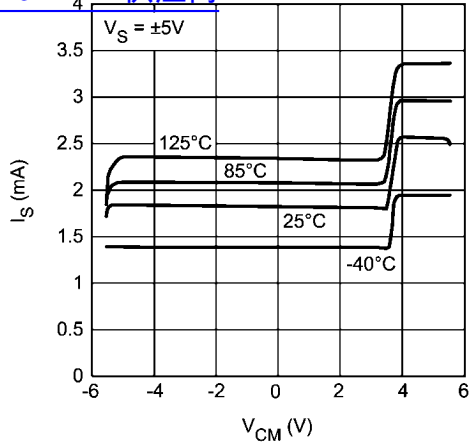
I_S vs. V_{CM} (LM7322) 查询"LM7321MA"供应商
