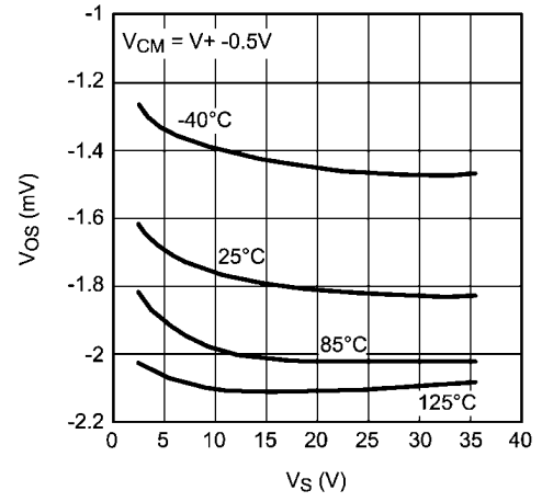
V OS vs. V S (Unit 3)
