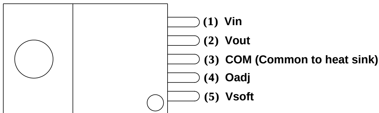
(TO-220-5)
