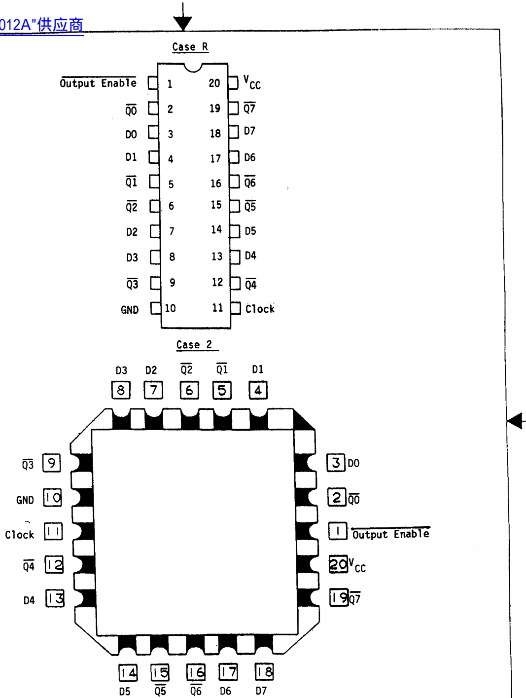
FIGURE 1. Terminal connections
