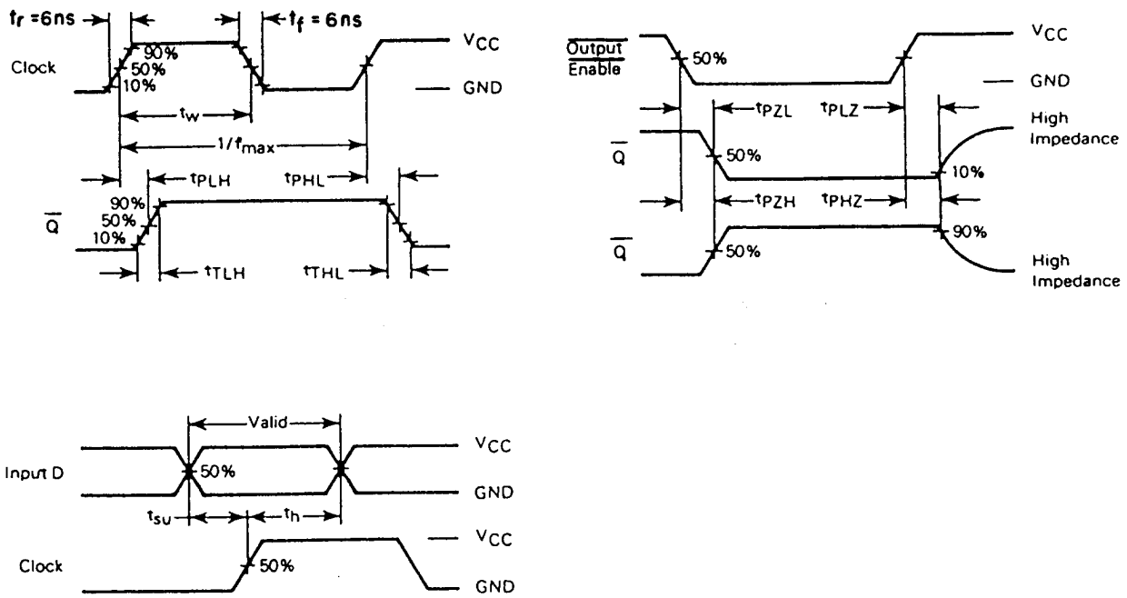
FIGURE 4. Switching waveforms.
