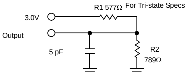
Figure 4. AC Test Loads
