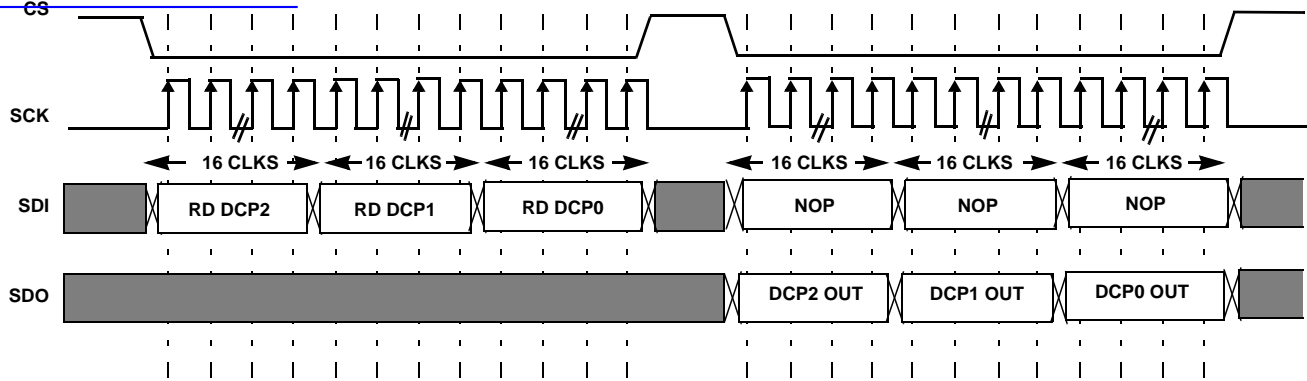
FIGURE 21. DAISY CHAIN READ SEQUENCE OF N = 3 DCP
