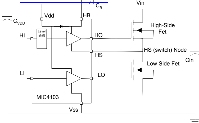
Figure 11. Synchronous Buck Converter Power Stage
