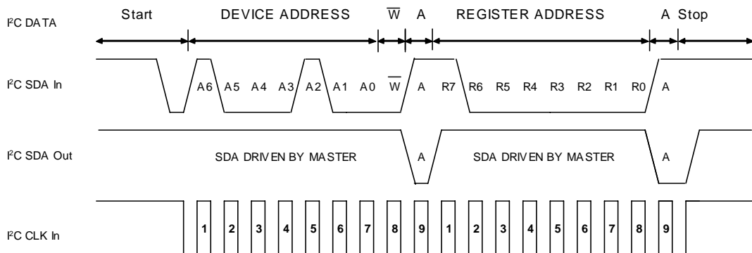
FIGURE 3. I²C SYNC_I²C TIMING DIAGRAM SAMPLE
