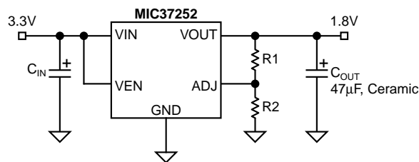
Adjustable Regulator
