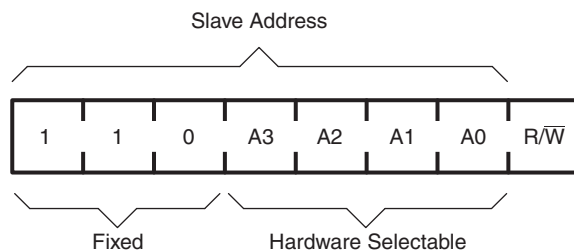
Figure 5. Slave Address
