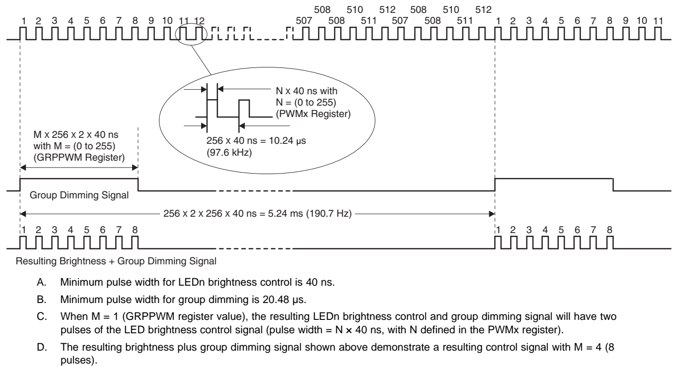
Figure 9. Brightness and Group Dimming Signals
