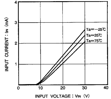
Figure 14 Input current - input voltage characteristic (BA12002)
