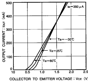
Fig. 12 Output current - voltage characteristic between collector and emitter
