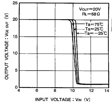
Fig.17 Output current - input voltage characteristics (BA12002)
