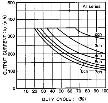
Fig. 7 Output conditions (1)
