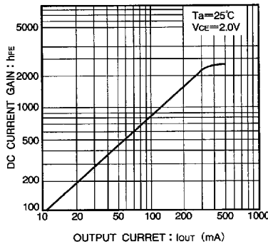
Fig. 10 DC current gain-output current characteristic
