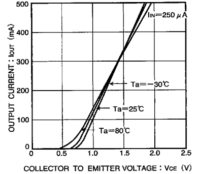
Fig. 11 Output current - voltage characteristic between collector and emitter
