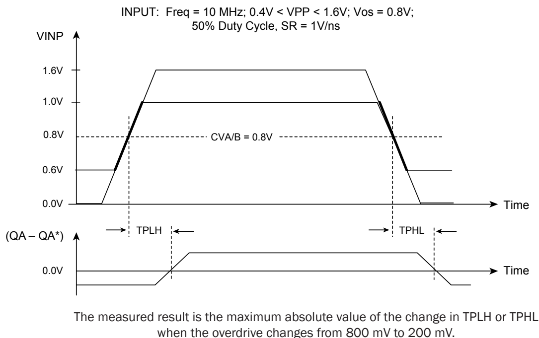
Figure 4. Comparator Dispersion: Overdrive Measurement Definition
