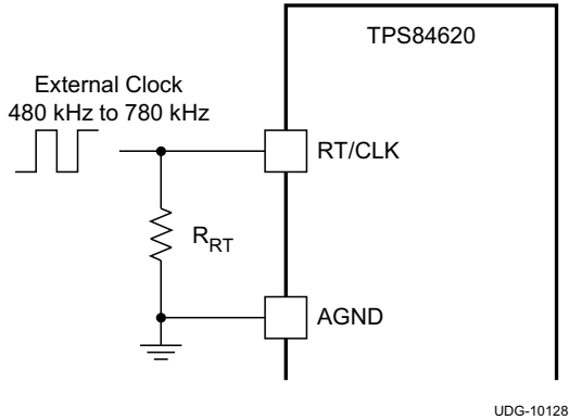
Figure 36. CLK/RT Configuration
