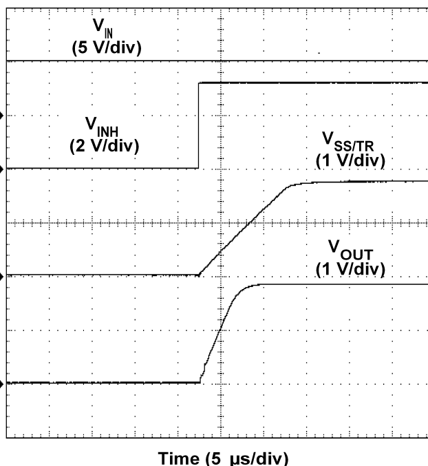
Figure 32. Inhibit Turn-On
