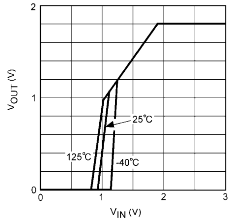
Turn-on Characteristics
