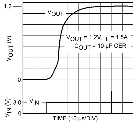
Turn-on Time
