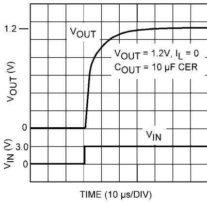
Turn-on Time
