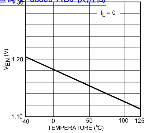
V_{EN} vs Temperature 查询"LP38500-ADJ"供应商
