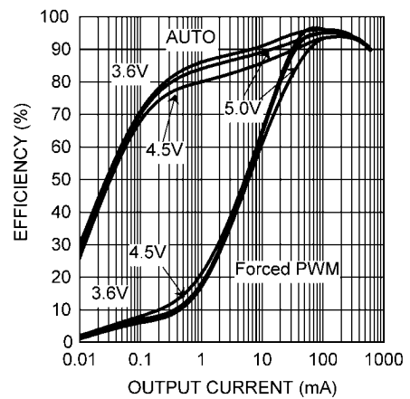
Efficiency vs. Output Current (V OUT = 3.3V, L = 2.2 μH)
