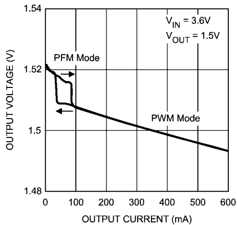
Output Voltage vs. Output Current (V OUT = 1.5V)
