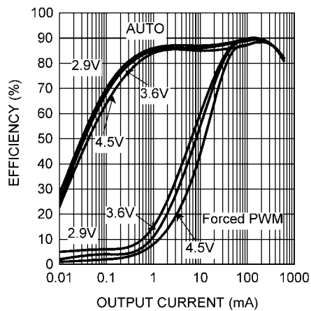
Efficiency vs. Output Current (V OUT = 1.5V, L = 2.2 μH)
