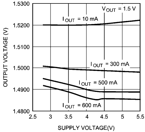
Output Voltage vs. Supply Voltage 查询"LM3676SD-1.5"供应商 (V OUT = 1.5V)
