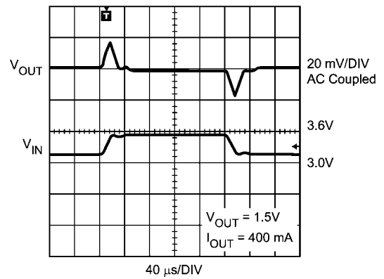
Line Transient Response V OUT = 1.5V (PWM Mode)
