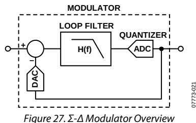
Figure 27. \Sigma - \Delta Modulator Overview
