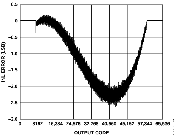
Figure 19. INL with f_{IN} = 2.4 \text{ MHz}
