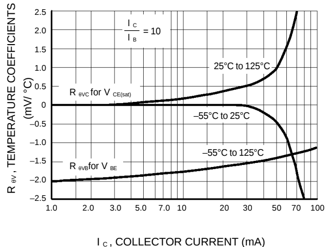
Figure 4. Temperature Coefficients
