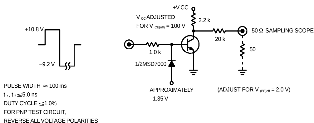
Figure 8. Switching Time Test Circuit
