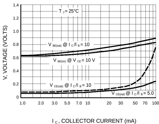
Figure 3. "On" Voltages
