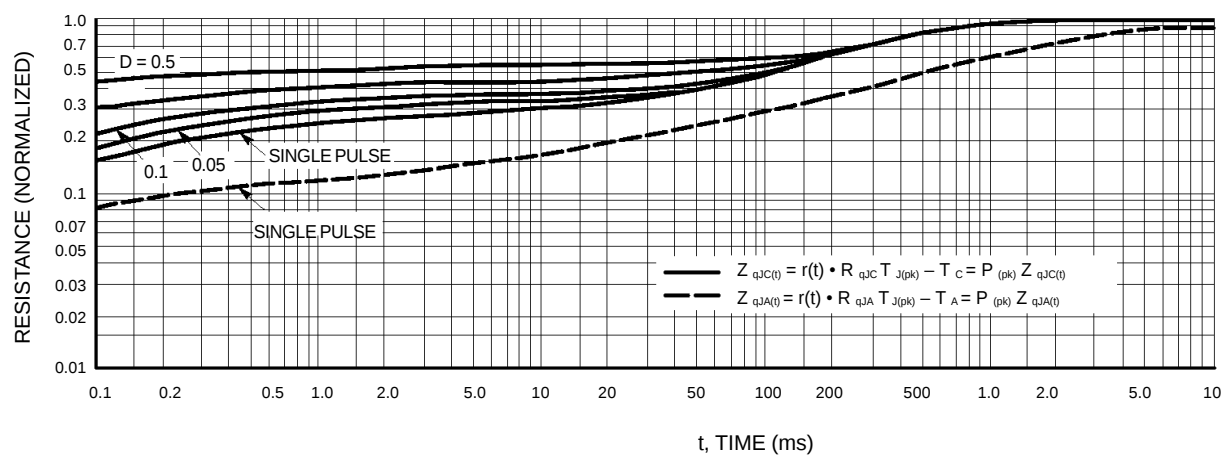
Figure 9. Thermal Response
