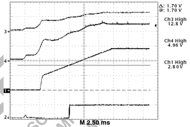
Figure 17. Implementing Power Good with the CS5158
