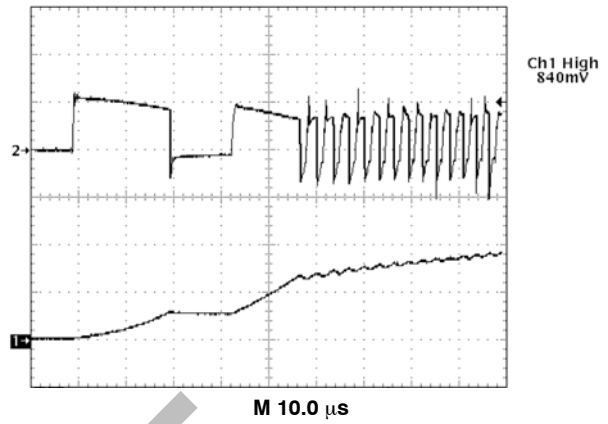
Figure 6. CS5158 Demonstration Board Enable Startup Waveforms
