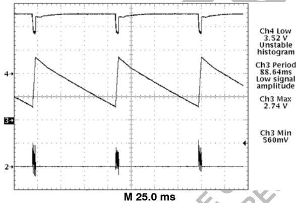
Figure 12. CS5158 Demonstration Board Hiccup Mode Short Circuit Protection. Gate Pulses are Delivered While the Soft Start Capacitor Charges, and Cease During Discharge
