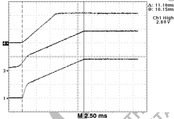
Figure 4. CS5158 Demonstration Board Startup in Response to Increasing 12 V and 5.0 V Input Voltages. Extended Off Time is Followed by Normal Off Time Operation when Output Voltage Achieves Regulation to the Error Amplifier Output.
