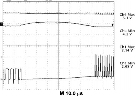
Figure 14. OVP Response to an Input-to-Output Short Circuit by Immediately Providing 0% Duty Cycle, Crow-Barring the Input Voltage to Ground
