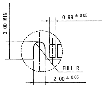
Detail "X"
