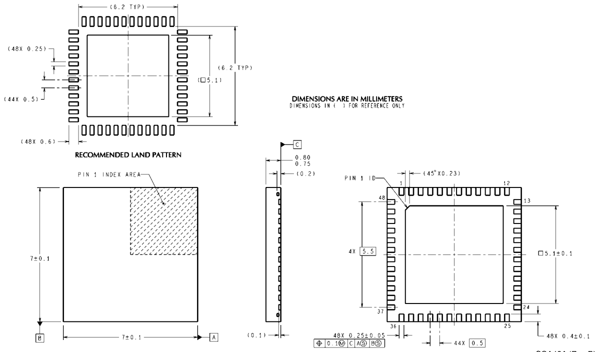
48-Lead QFN Plastic Quad Package NS Package Number SQA48A
