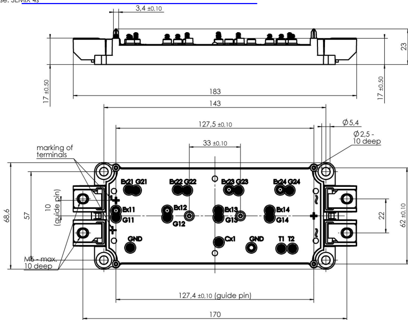
Case SEMiX 4s
