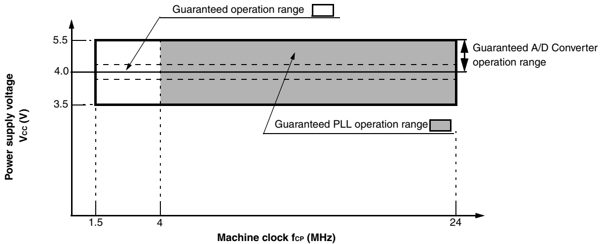
Guaranteed operation range of MB90340E series
