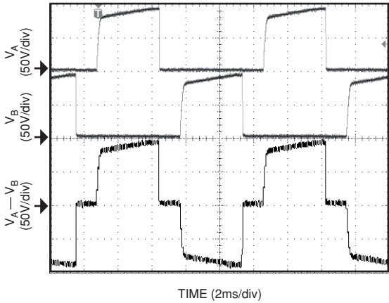
Figure 7. Typical EL Driver for 2in 2 Lamp with 560μH inductor
