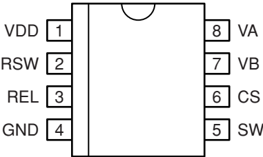
8-Pin MSOP Package (MM)
