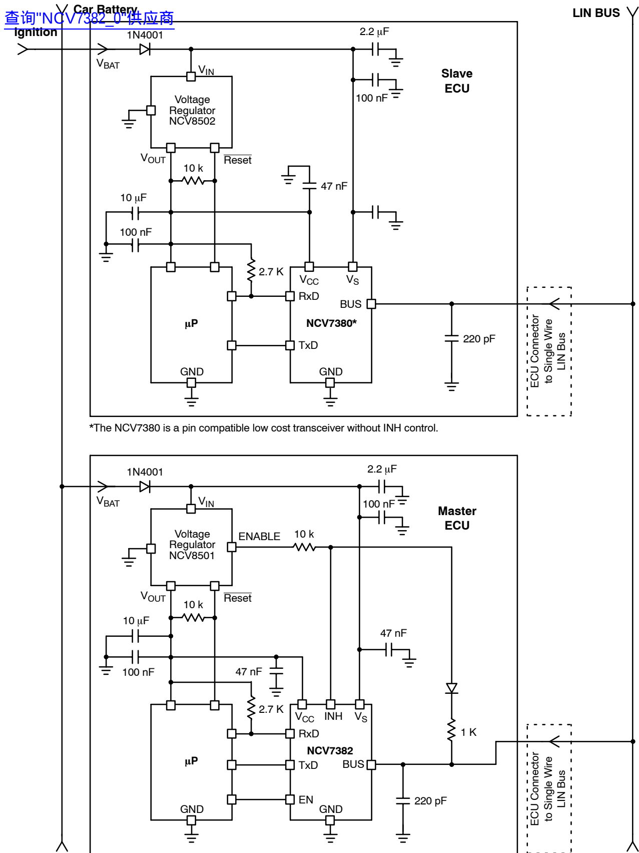
Figure 10. Application Circuitry
