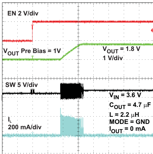
Time Base - 20 μs/div
