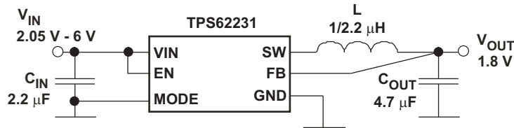
Figure 51. TPS62231 1.8V Output
