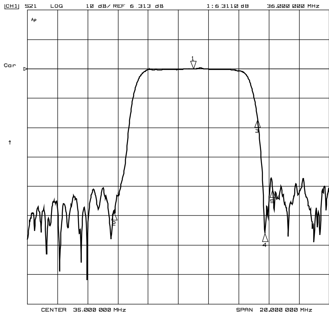
Amplitude Response [Channel2-BW=7.4MHz] (10dB/div)
