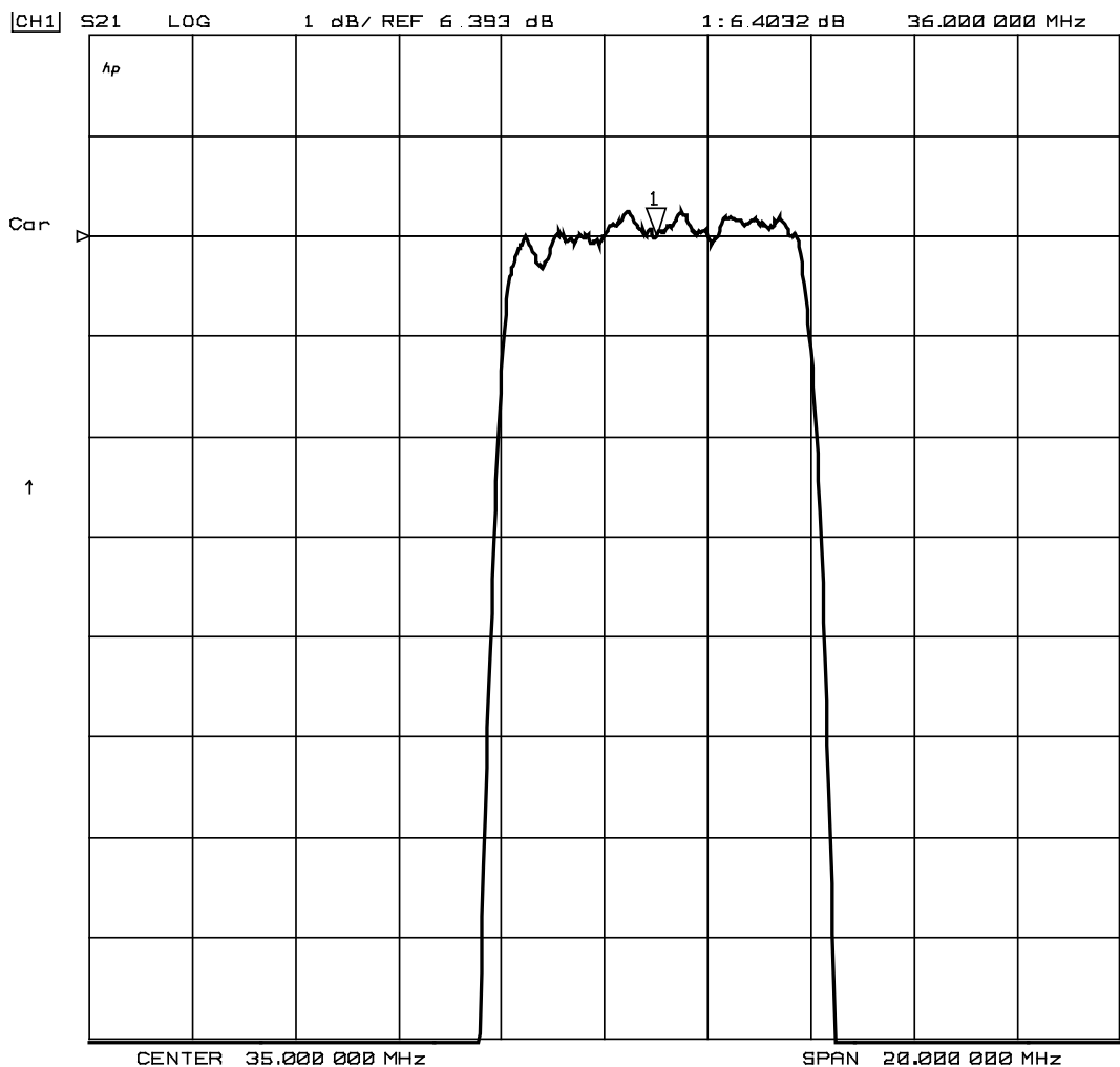
Amplitude Response [Channel1-BW=6.4MHz] (1dB/div)
