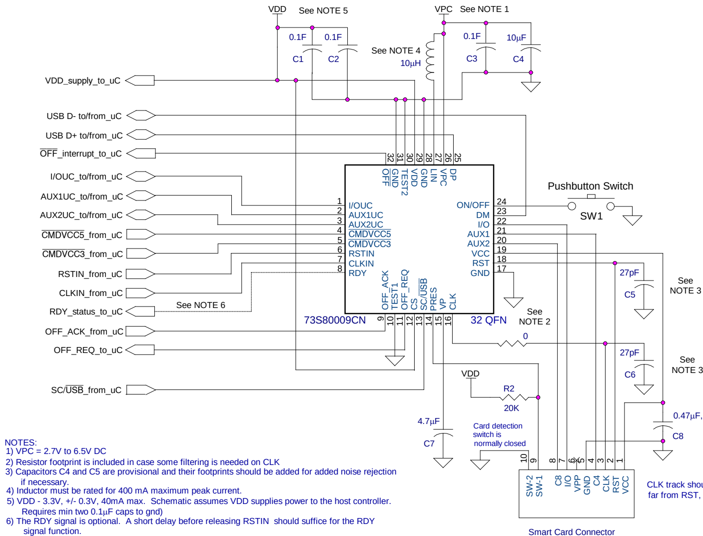
Figure 3: Typical 73S8009CN Application Schematic with a Main System Switch
