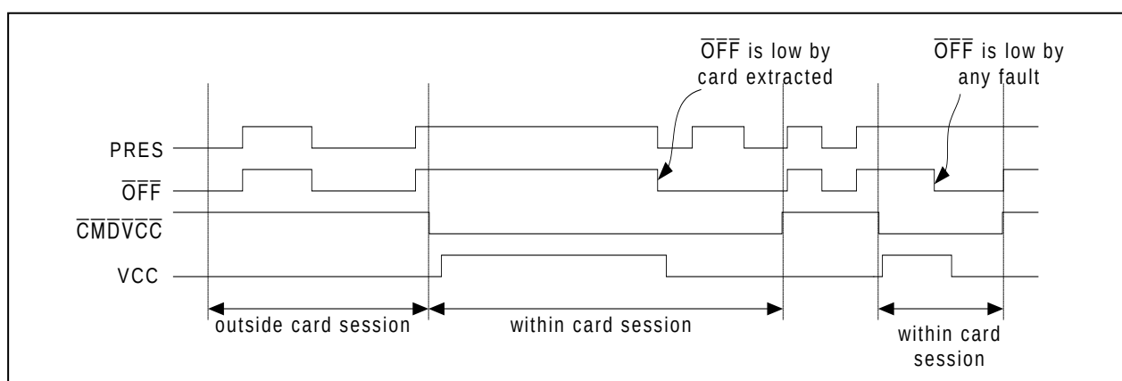
Figure 7: \overline{\text{OFF}} Activity
