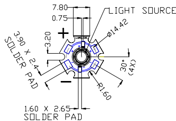
Lambertian
