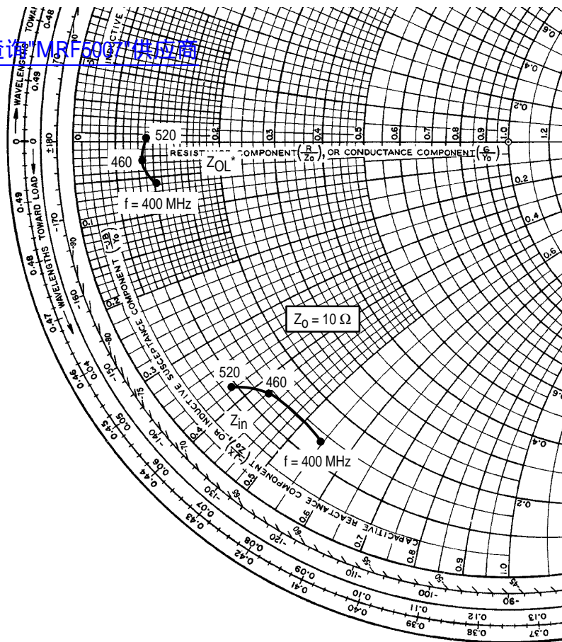
Figure 11. Series Equivalent Input and Output Impedance
