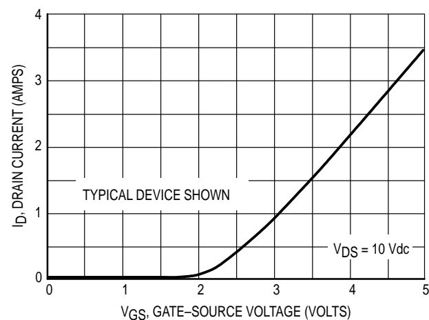
Figure 7. Drain Current versus Gate Voltage
