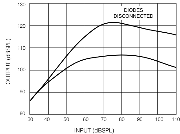
Fig. 7 I/O Characteristics
