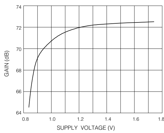
Fig. 12 Gain vs Supply Voltage
