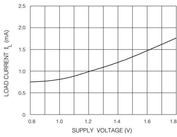
Fig. 11 Load Current vs Supply Voltage
