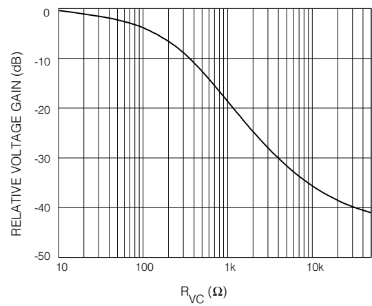
Fig. 8 Relative Voltage Gain vs Volume Control Resistance
