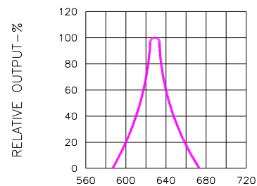
Fig.2 SPECTRAL RESPONSE
