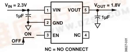
Figure 1. TSOT ADP151 with Fixed Output Voltage, 1.8 V
