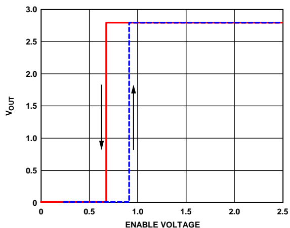
Figure 28. ADP151 Typical EN Pin Operation
