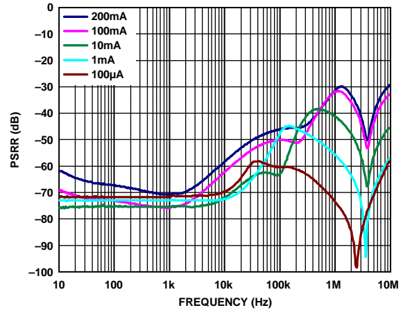
Figure 15. Power Supply Rejection Ratio vs. Frequency, V_{OUT} = 1.2 V , V_{IN} = 2.2 V
