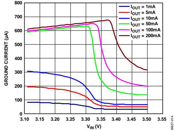
Figure 14. Ground Current vs. Input Voltage (in Dropout)
