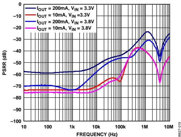
Figure 19. Power Supply Rejection Ratio vs. Frequency at Various Voltages and Load Currents, V_{OUT} = 2.8V
