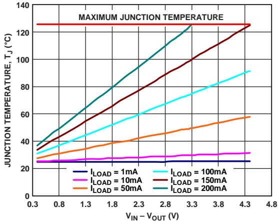
Figure 37. WLCSP 500 mm 2 of PCB Copper, T_A = 25^\circ\text{C}
