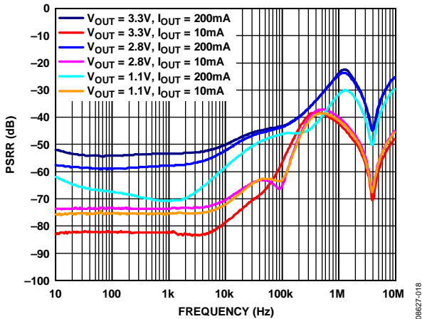
Figure 18. Power Supply Rejection Ratio vs. Frequency at Various Output Voltages and Load Currents, V_{OUT} - V_{IN} = .0.5V , except for V_{OUT} = 1.1V , V_{IN} = 2.2V
