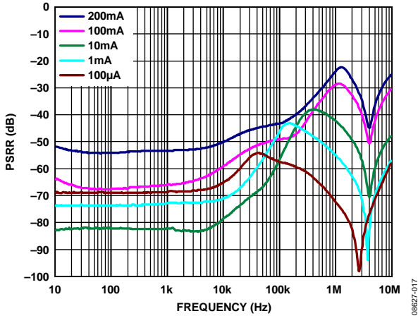
Figure 17. Power Supply Rejection Ratio vs. Frequency, V_{OUT} = 3.3V , V_{IN} = 3.8V
