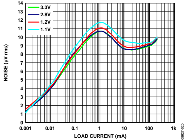
Figure 20. Output Noise vs. Load Current and Output Voltage, V_{IN} = 5V , C_{OUT} = 1\mu F
