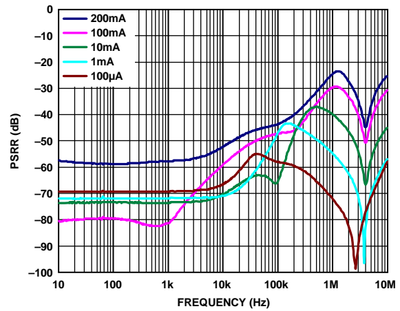
Figure 16. Power Supply Rejection Ratio vs. Frequency, V_{OUT} = 2.8 V , V_{IN} = 3.3 V
