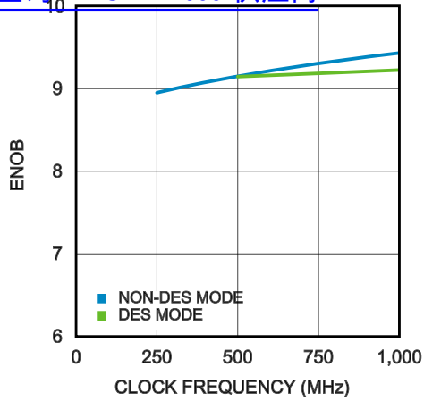
ENOB vs. CLOCK FREQUENCY (ADC12D1000) 查询"ADC12D1000"供应商
