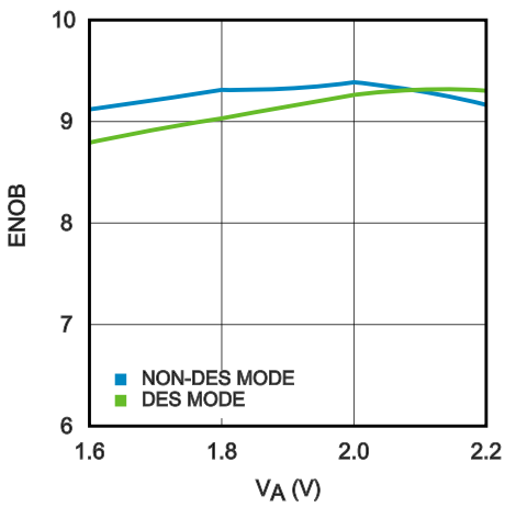
ENOB vs. SUPPLY VOLTAGE (ADC12D1000)
