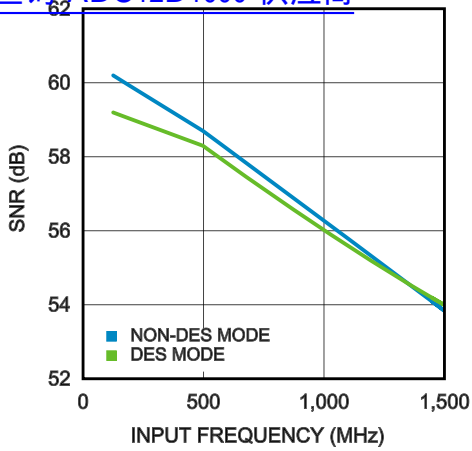
SNR vs. INPUT FREQUENCY (ADC12D1000) 查询"ADC12D1000"供应商
