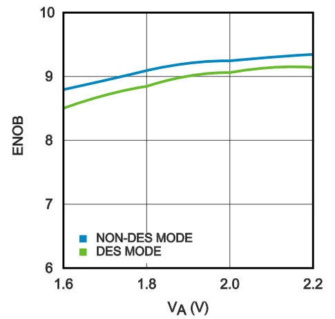
ENOB vs. SUPPLY VOLTAGE (ADC12D1600)
