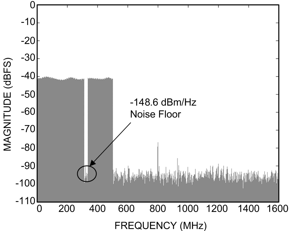
Wideband Performance
