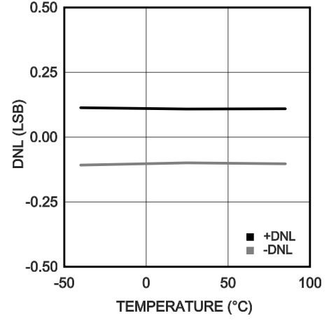
DNL vs. TEMPERATURE (ADC12D1600)
