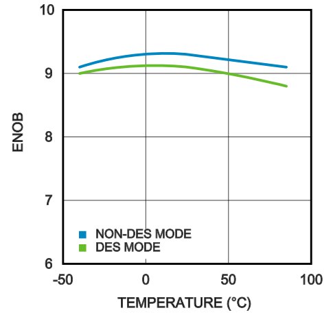
ENOB vs. TEMPERATURE (ADC12D1600)
