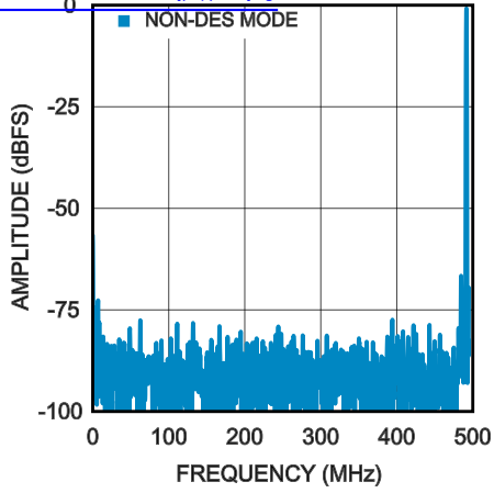
SPECTRAL RESPONSE AT FIN = 498 MHz (ADC12D1000) 查询"ADC12D1000"供应商
