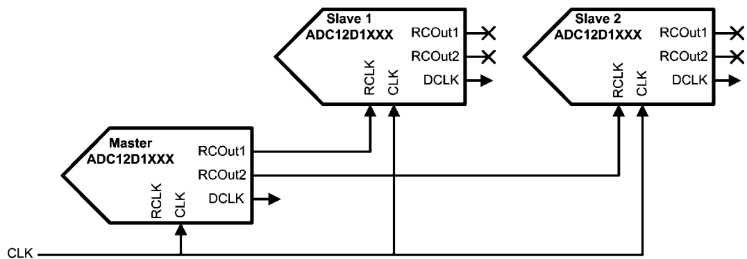
FIGURE 18. AutoSync Example
