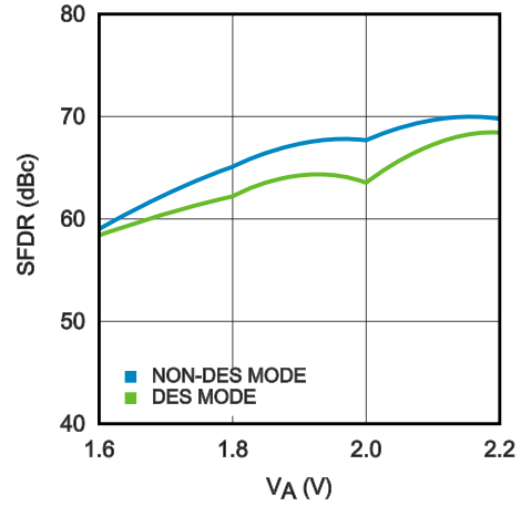
SFDR vs. SUPPLY VOLTAGE (ADC12D1600)
