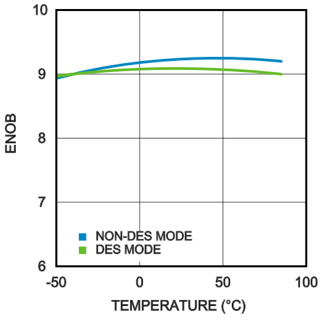
ENOB vs. TEMPERATURE (ADC12D1000)
