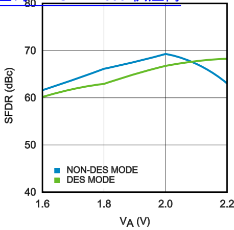
SFDR vs. SUPPLY VOLTAGE (ADC12D1000) 查询"ADC12D1000"供应商
