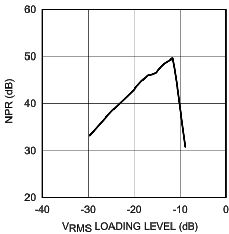
NPR vs. RMS NOISE LOADING LEVEL (ADC12D1000)
