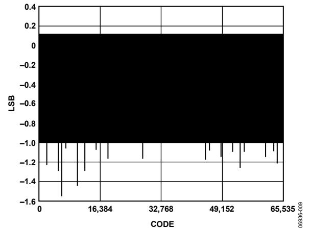
Figure 9. AD9783 DNL, T_A = 25^\circ\text{C} , FS = 20\text{ mA}
