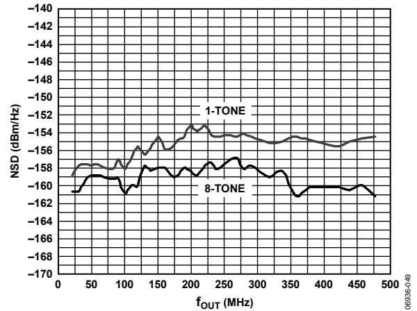
Figure 49. AD9780 One-Tone, Eight-Tone NSD vs. f_{OUT} in Baseband and Mix Modes, at 500 MSPS, FS = 20 mA
