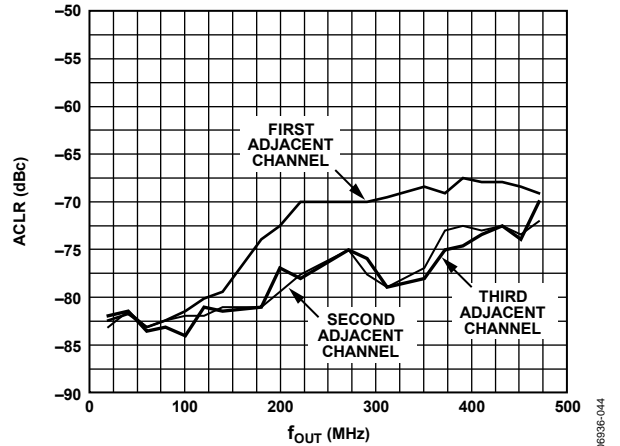
Figure 44. AD9781 ACLR for One-Carrier W-CDMA Baseband and Mix Modes, at 491.52 MSPS, FS = 20\text{ mA}
