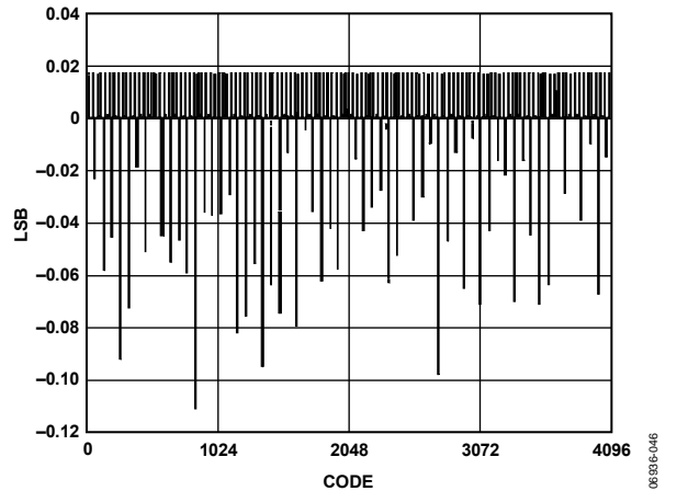
Figure 46. AD9780 DNL, FS = 20\text{ mA}
