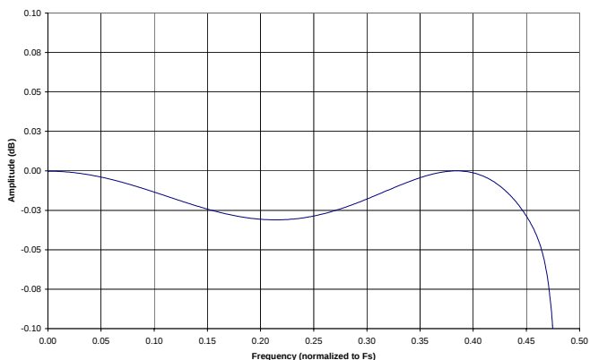
Figure 30. Single-Speed Mode Passband Ripple
