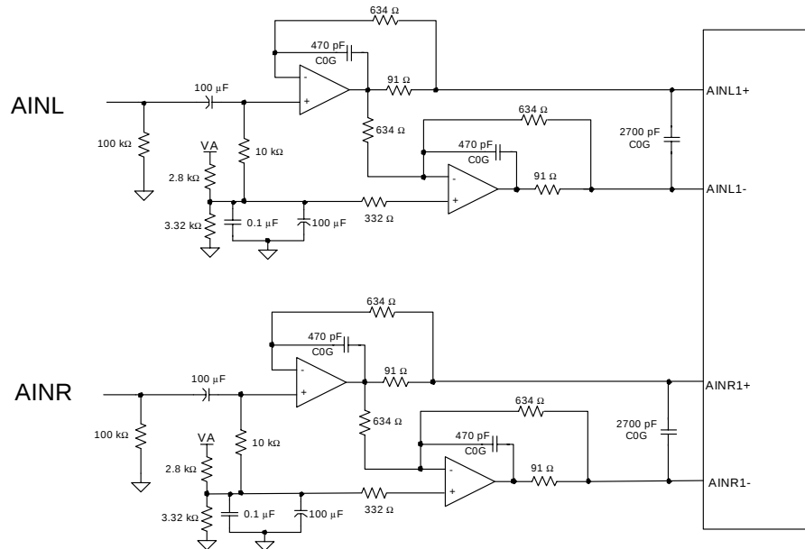
Figure 24. Recommended Analog Input Buffer
